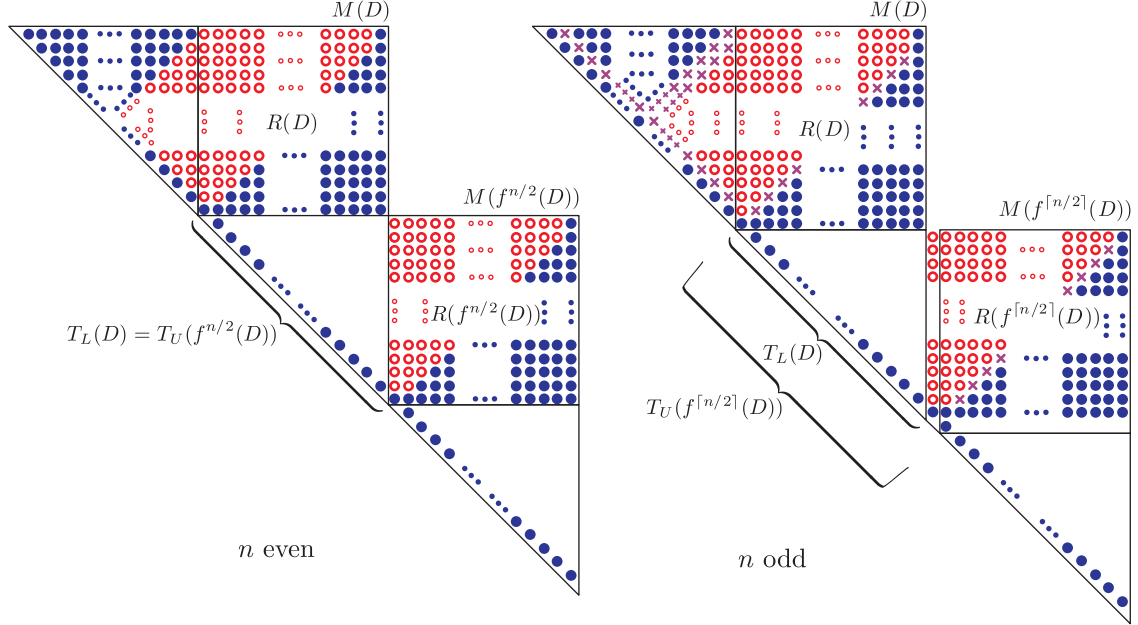
Figure 9: The lower triangle T_L(D) versus the upper triangle T_U(f^{\lceil n/2 \rceil}(D)) for even and odd n in the proof of Theorem 23.
