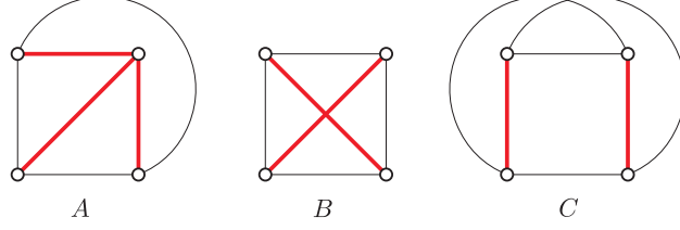
Figure 1: The three non plane-homeomorphic good drawings of K_4 , with 3, 2, and 2 separations. The edge of each separation is shown bold.
