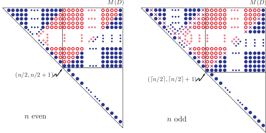
Figure 8: The upper triangle T_U(D) for even and odd n in the proof of Theorem 23.
