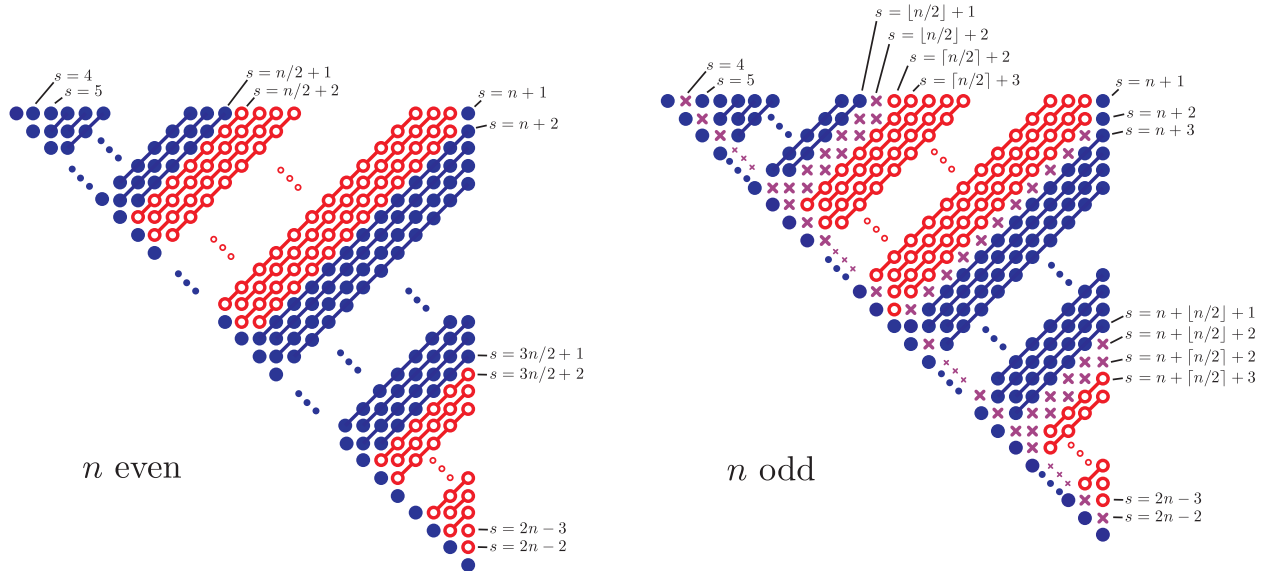
Figure 6: The even and odd cases in Theorem 23. The crosses in the odd case represent points whose color is not fixed.
