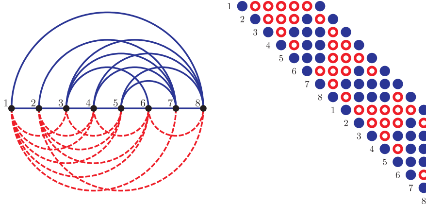
Figure 3: A 2-page drawing of K_8 and its strip diagram.
