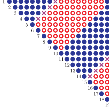
Figure 10: The 2^8 crossing optimal drawings (only 2^7 non-equivalent) for n = 19 in Theorem 27. They are obtained by assigning arbitrary colors to the crosses in this matrix.
