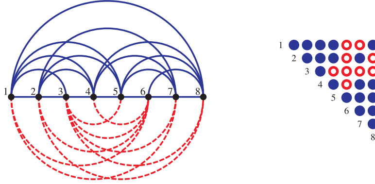
Figure 4: A 2-page book drawing of K_8 with four 0-edges (namely 17, 18, 27, and 28) and four 1-edges (namely 15, 16, 38, and 48). This shows that the inequality E_{\leq k}(D) \geq 3\binom{k+2}{2} , which holds for every geometric drawing D of K_n , does not necessarily hold if D is a topological drawing.
