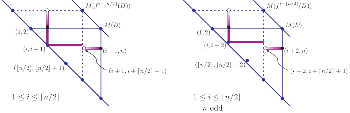
Figure 5: A halving line in a drawing equivalent to D seen in the matrix M(D) .
